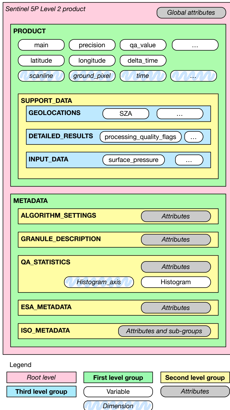
Figure 5: Graphical description of the generic structure of a Level 2 file. The elements labeled as a dimension are coordinate variables. See section 8 for a full description.
